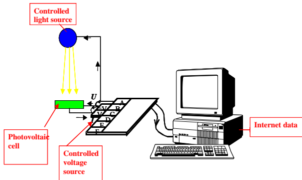
Figure 2. The schematic representation of the server of the remote experiment “Photovoltaic cell” using the system ISES http://kdt-4.karlov.mff.cuni.cz/vacharakteristika_2_en.html
