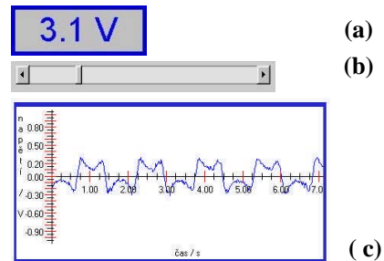
Figure 3. Examples of modular Java applets from ISES WEB Control kit as building tools and blocks for remote experiments web control pages (a) display, (b) control slide, (c) graph for data presentation.
